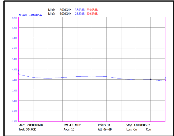
Noise Figure(2-4GHz)
