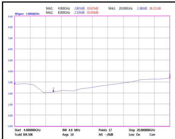
Noise Figure(4-20GHz)
