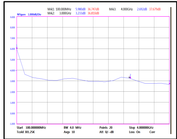
Noise Figure(0.1-4GHz)
