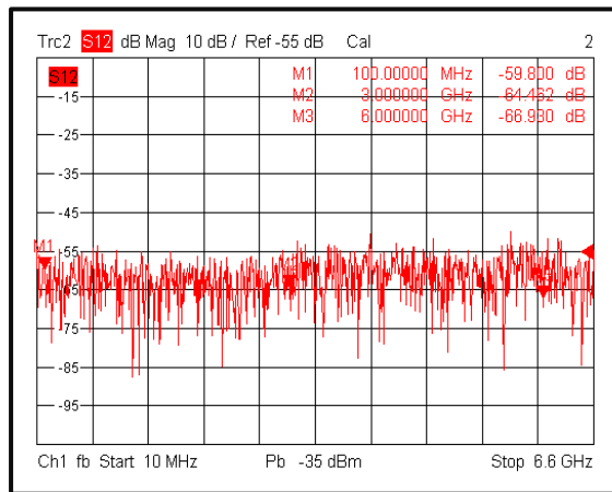
Isolation@+85°C
